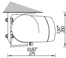
Ceiling installation
