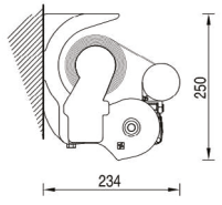
Ceiling installation
