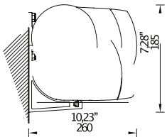
Wall installation
